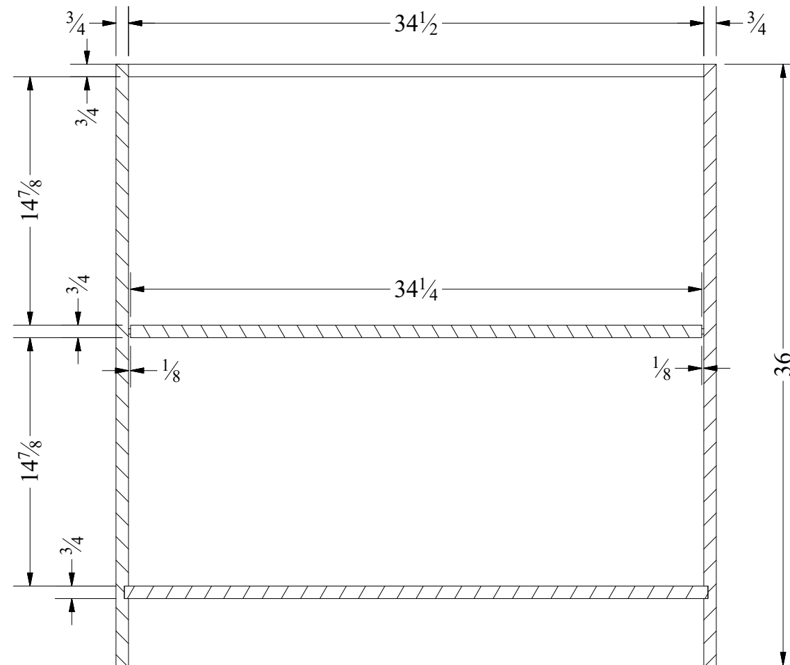
SECTION B-B
